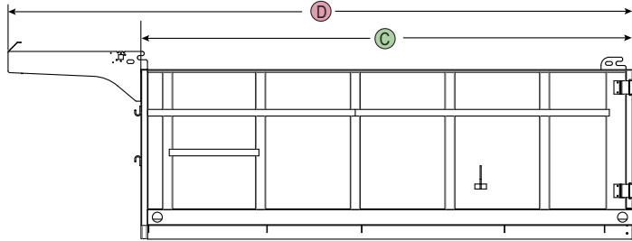
Roadside View (40" cab guard shown)
