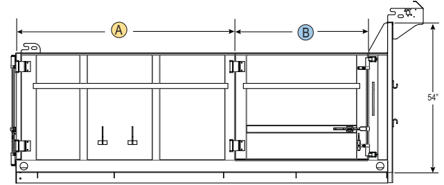
Curbside View (12" cab guard shown)
