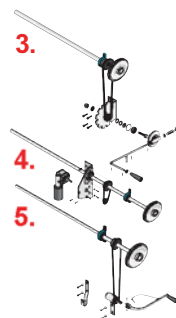
Twin Cable Top Slider
