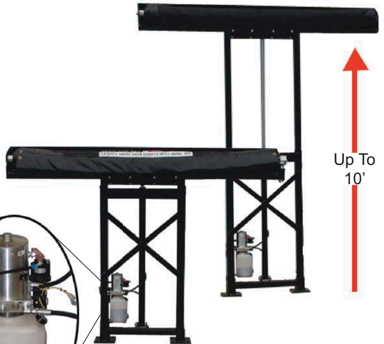
Part #501-9958
