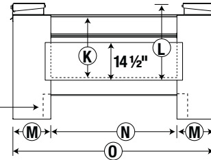
Single Wheel Rear View
